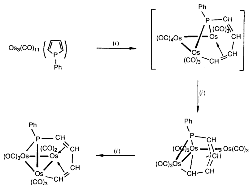
Scheme 1 (i) Refluxing octane
